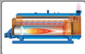
Typical 3-pass wetback boiler.
