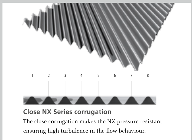
NT Series plate corrugation
